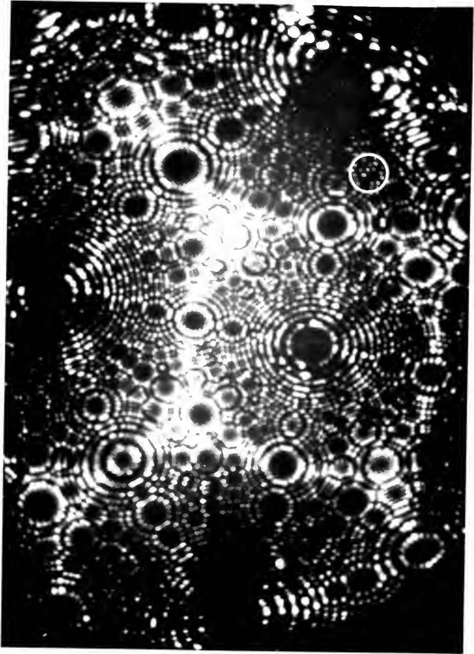
Figure 38.--(b) Same specimen after removing a single (002) plane. Note that the void is somewhat larger.
